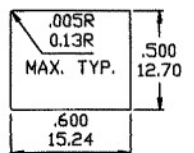
PANEL MOUNTING
